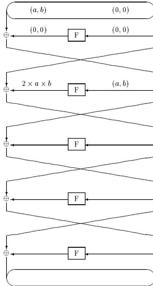
Fig. 1. A second order differential of a five round Feistel cipher
