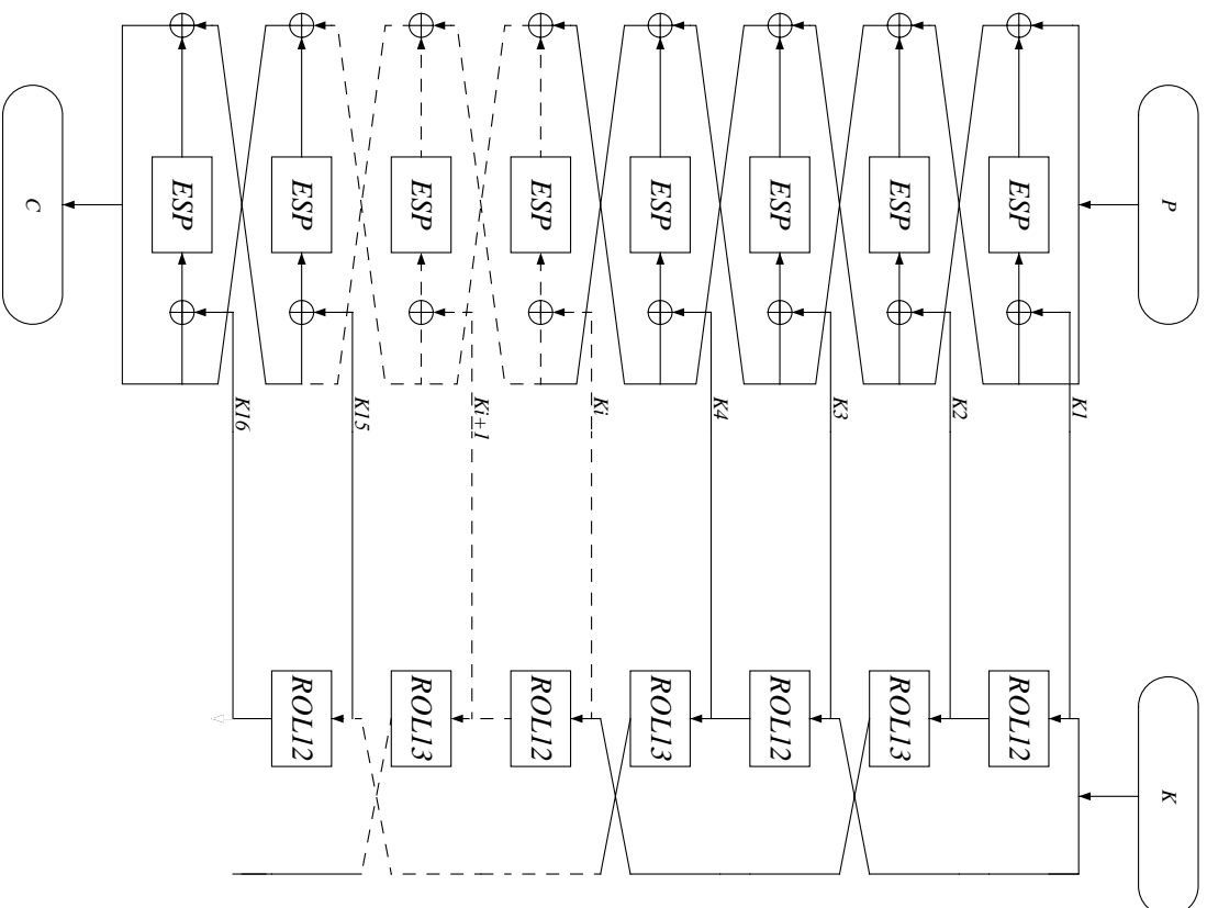
Figure 2. Outline of LOKI191.
